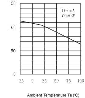
Fig.8 Relative Current Transfer Ratio vs. Ambient Temperature
